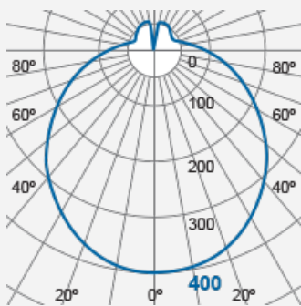
Integrated LED Luminaire FIB70000v1
