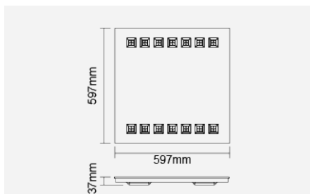
Integrated LED Luminaire FPL62400v0
