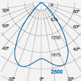
Integrated LED Luminaire FPL62400v0
