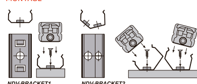
NDV-BRACKET1 Mounting clip
