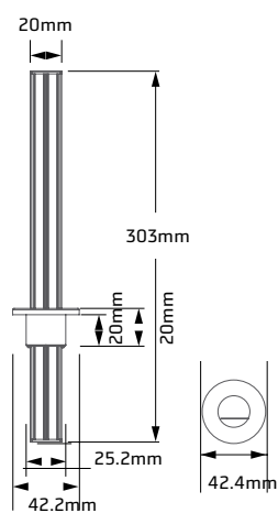
MNR-Rail extrusion pole
